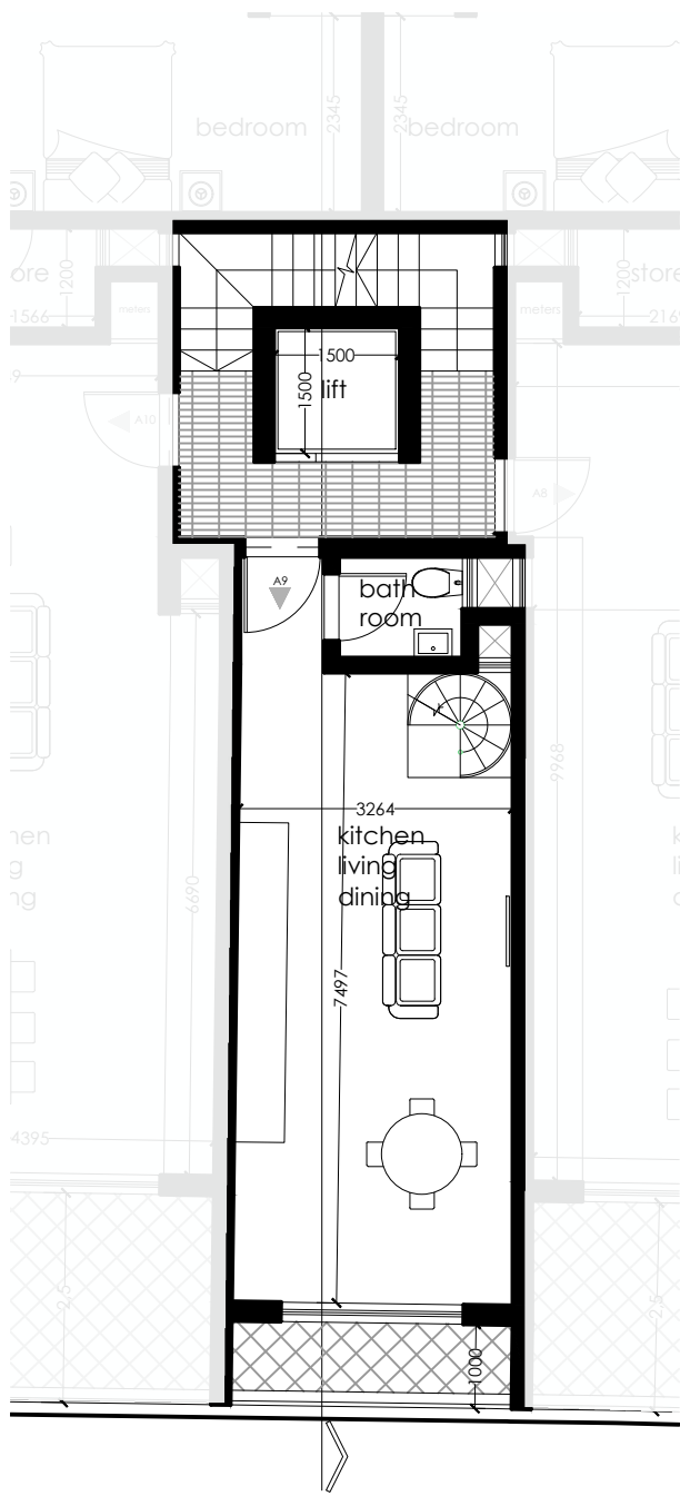
Fourth Floor Level - Part-Plan
