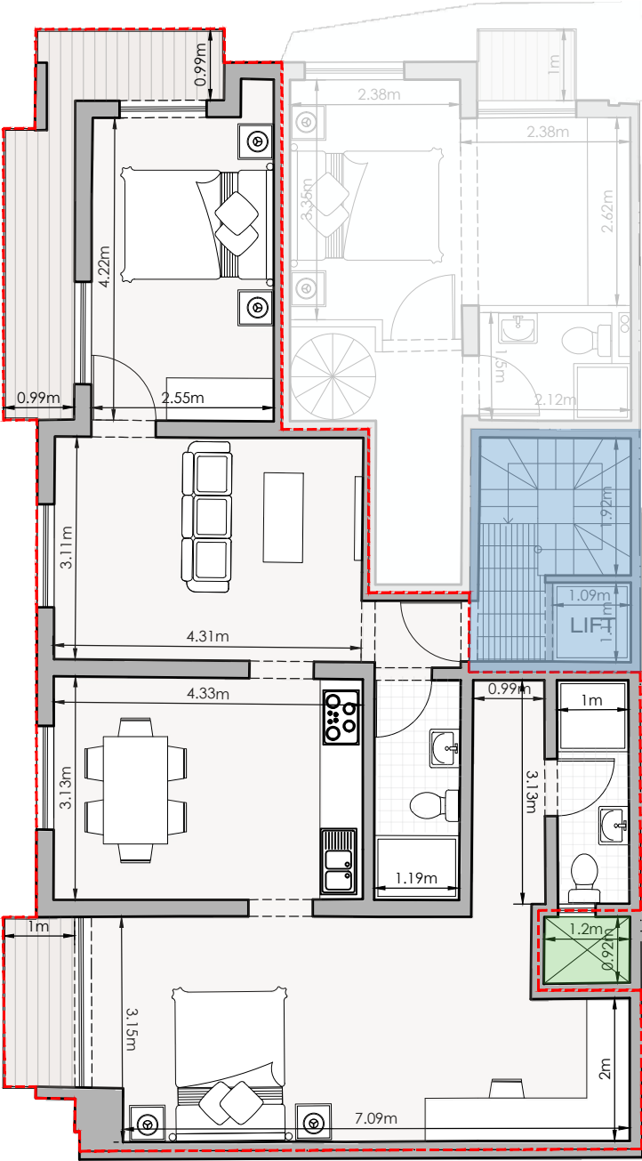
Second Floor Level Scale:- 1:100
